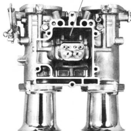
Starter Jet
